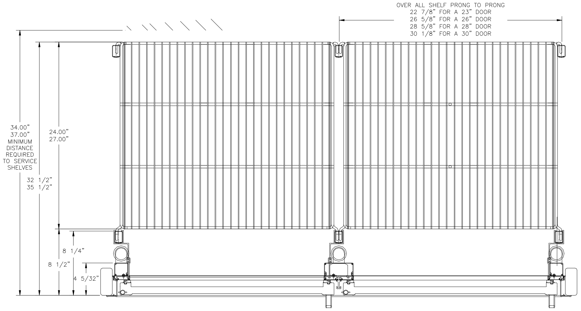
LEGACY SERIES OVERALL SHELF DIMENSIONS
