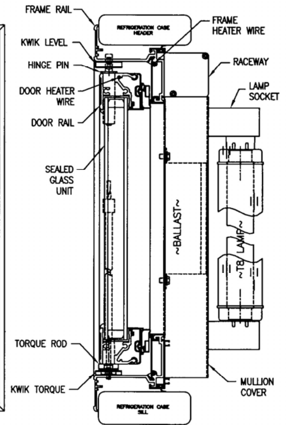
LEGACY SERIES SIDE CROSS SECTION
