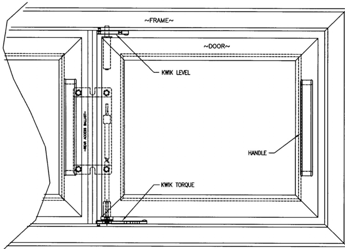
LEGACY SERIES FRONT ELEVATION
