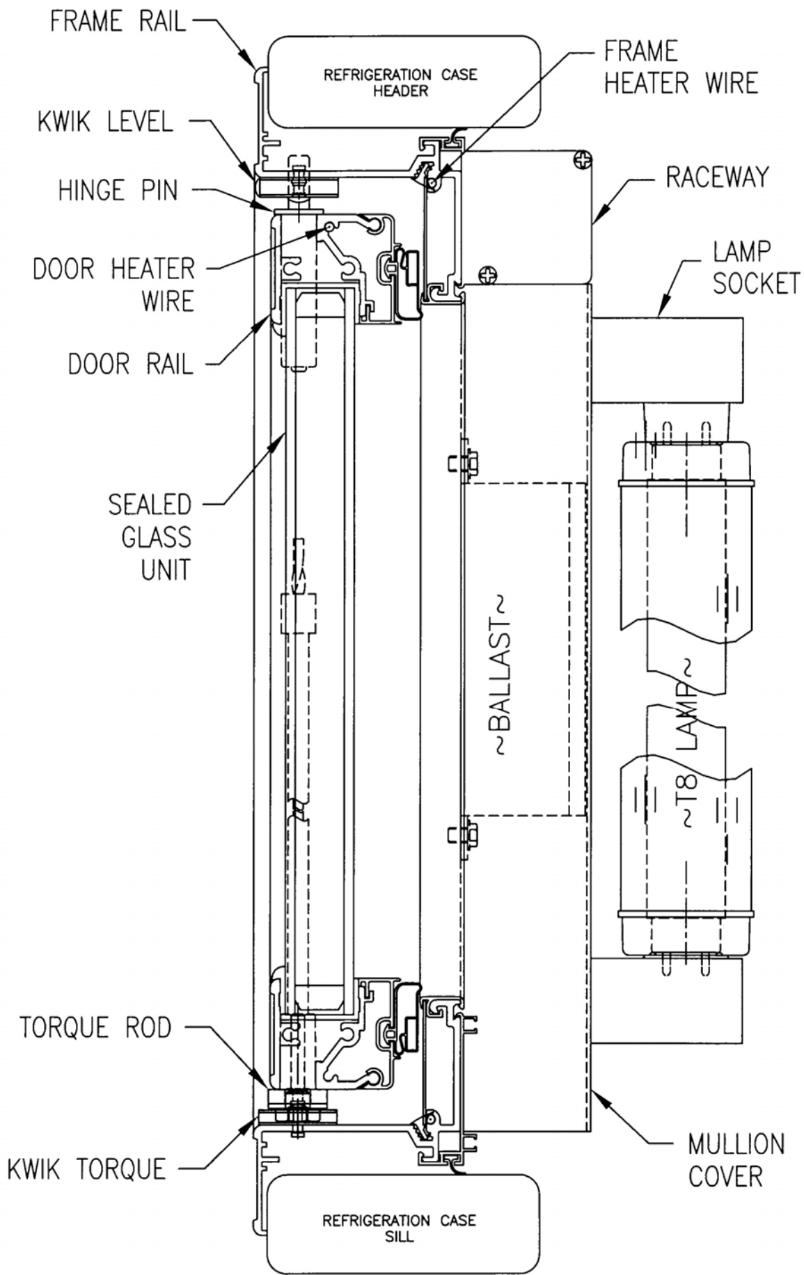
LEGACY SERIES SIDE CROSS SECTION
